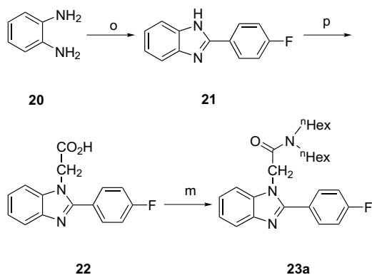
Scheme 3. Reagents and conditions: (o) 4-F- \text{Ph}\text{-CO}_2\text{H} , \text{PPA} ; (p) \text{BrCH}_2\text{CO}_2\text{H} , \text{KOH} , \text{DMSO} ; (m) \text{ClCO}_2\text{Et} , (n\text{-Hex})_2\text{NH} , \text{Et}_3\text{N} , \text{THF} . Method G: o, p, m.
