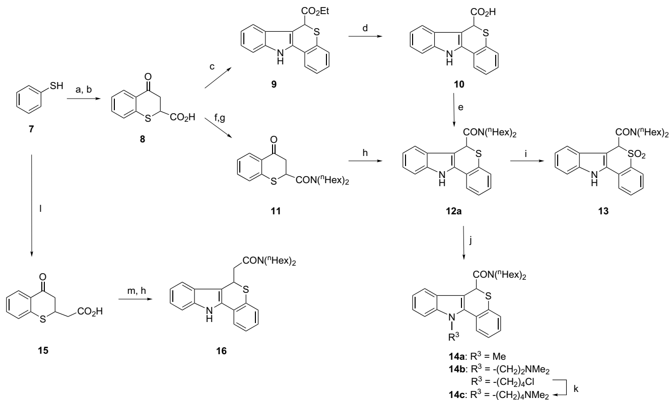
Scheme 1. Reagents and conditions: (a) furan-2,5-dione, \text{Et}_3\text{N} , toluene; (b) \text{AlCl}_3 , \text{CH}_2\text{Cl}_2 ; (c) \text{PhNHNH}_2 , \text{H}_2\text{SO}_4 , \text{EtOH} ; (d) \text{KOH} , \text{EtOH} , \text{H}_2\text{O} ; (e) n\text{-Hex}_2\text{NH} , \text{EDC}\cdot\text{HCl} , \text{HOBT} , \text{CH}_2\text{Cl}_2 ; (f) \text{SOCl}_2 , \text{PhH} ; (g) n\text{-Hex}_2\text{NH} , \text{Et}_3\text{N} , \text{CH}_2\text{Cl}_2 ; (h) \text{PhNHNH}_2 , \text{ZnCl}_2 , heat; (i) m\text{CPBA} , \text{CH}_2\text{Cl}_2 ; (j) \text{R}^3\text{Cl} or \text{R}^3\text{Br} , \text{NaH} , \text{DMF} ; (k) \text{Me}_2\text{NH} , \text{MeOH} ; (l) pent-2-enedioic acid, \text{Et}_3\text{N} ; (m) \text{ClCO}_2\text{Et} , n\text{-Hex}_2\text{NH} , \text{Et}_3\text{N} , \text{THF} . Method A: a, b, c, d, e; method B: a, b, f, g, h; method C: i; method D: j, k; method E: l, m, h.
