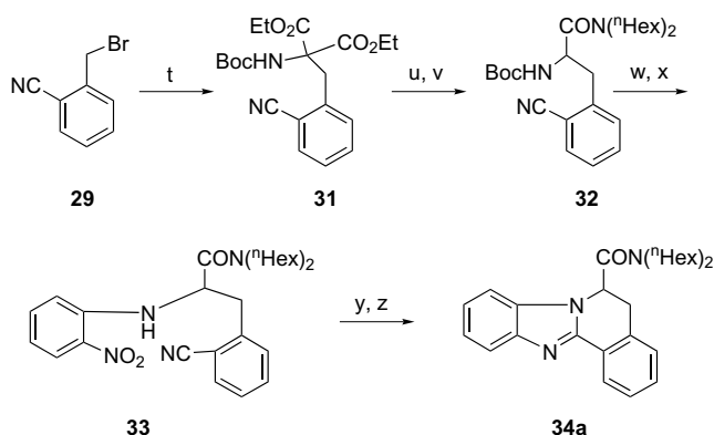
Scheme 5. Reagents and conditions: (t) \text{BocNHCH}(\text{CO}_2\text{Et})_2 , 30 , \text{EtONa} , \text{EtOH} ; (u) \text{NaOH} , \text{EtOH} , \text{H}_2\text{O} ; (v) (\text{n-Hex})_2\text{NH} , \text{EDC}\cdot\text{HCl} , \text{HOBt} , DMF; (w) \text{TFA} , \text{CH}_2\text{Cl}_2 ; (x) 2-fluoronitrobenzene, \text{K}_2\text{CO}_3 , DMF; (y) \text{H}_2 , \text{PtO}_2 , \text{MeOH} ; (z) \text{HCl} gas, \text{EtOH} . Method H: t–z.
