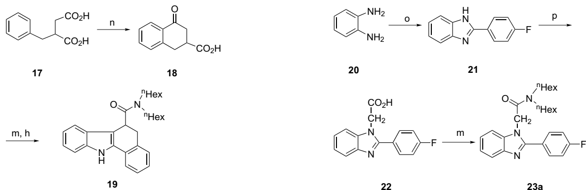
Scheme 2. Reagents and conditions: (n) \text{H}_2\text{SO}_4 ; (m) \text{ClCO}_2\text{Et} , (n\text{-Hex})_2\text{NH} , \text{Et}_3\text{N} , \text{THF} ; (h) \text{PhNHNH}_2 , \text{ZnCl}_2 , heat. Method F: n, m, h.
