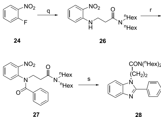
Scheme 4. Reagents and conditions: (q) \text{NH}_2\text{CH}_2\text{CH}_2\text{CON}(\text{n-Hex})_2 ( 25 ), \text{K}_2\text{CO}_3 , DMF; (r) \text{PhCOCl} , \text{Et}_3\text{N} , \text{CH}_2\text{Cl}_2 ; (s) \text{Fe} , \text{AcOH} . Method H: q, r, s.
